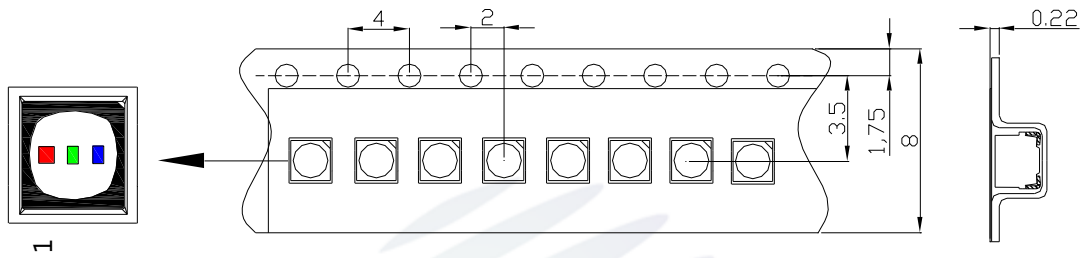
Fig.2-1 Carrier Tape Dimension
