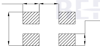
Fig.1-5 Soldering patterns
